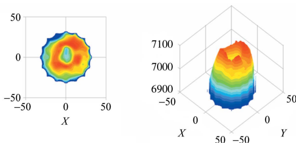
Figure 5 Measured angular distribution of the radiation from the 5 μm-thick Mo strip target. [To appear in black and white but colour online]
