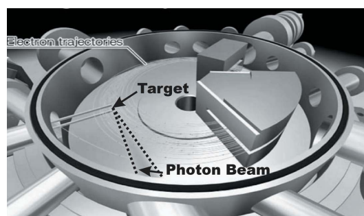
Figure 1 Each of the electrons circulating in MIRRORCLE passes through a small target many times, emitting a photon beam. The magnetic field is perpendicular to the circulation plane. [To appear in black and white but colour online]
