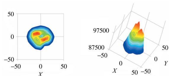
Figure 8 Angular distribution for the CNT yarn with a diameter of 15 μm. [To appear in black and white but colour online]
