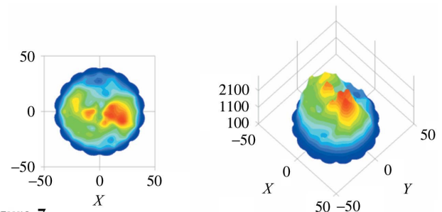
Figure 7 Angular distribution for the 385 nm-thick Al strip target. [To appear in black and white but colour online]
