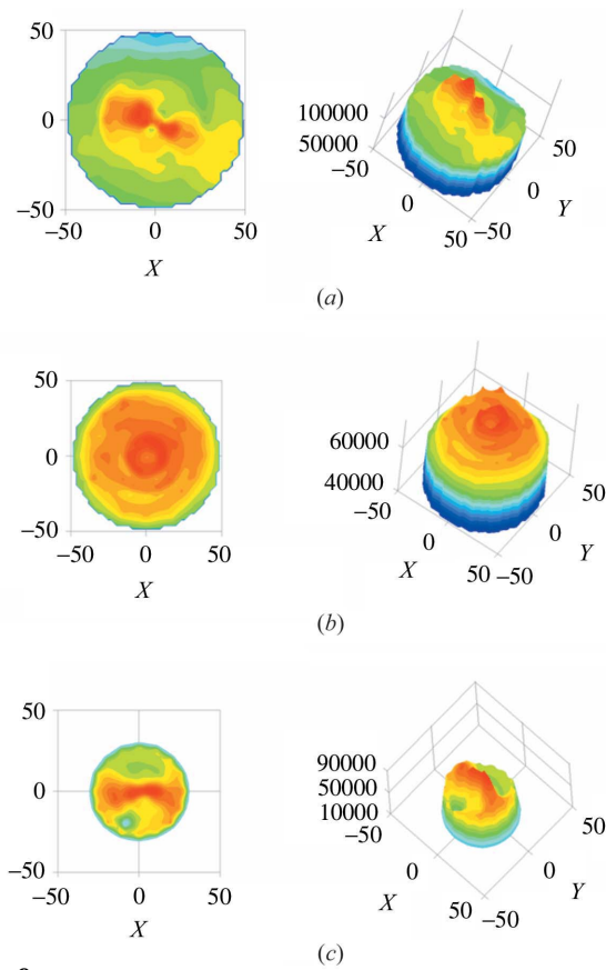
Figure 9 Angular distributions of the radiation from the 55 nm-thick DLC strip target. (a) Without Al filter. (b) With a 385 nm-thick Al filter in front of the PS. (c) The difference between the above two distributions. [To appear in black and white but colour online]
