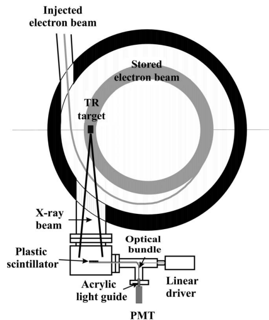
Figure 2 Set-up of our experiment for measurement of the emitted power from MIRRORCLE-6X with a TR target.
